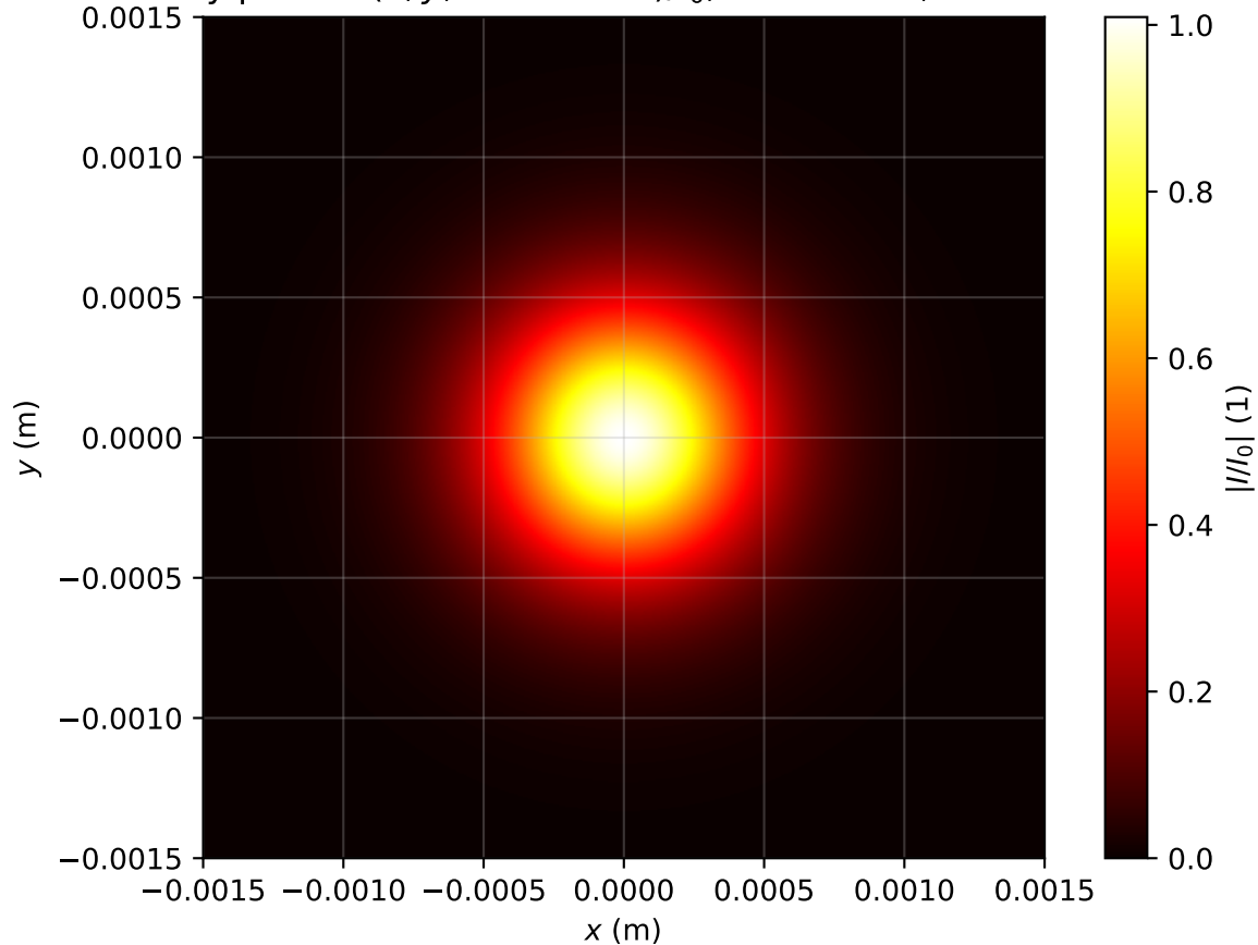
Intensity profile I(x, y, z = 1.274m)/I_0 , Pin=0.5Pcr, artificial time
